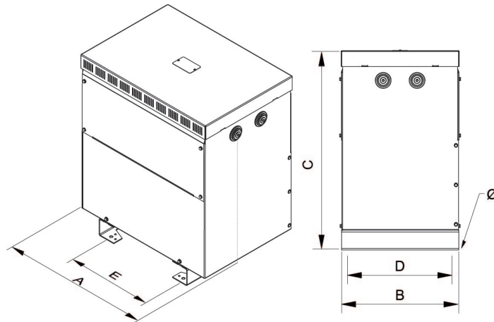
Dimensions (AxBxCxDxE): 595x415x708x375x350 mm 12Ø
