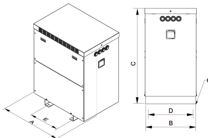
Dimensions (AxBxCxDxE): 985x675x1310x475x470 mm 18Ø
