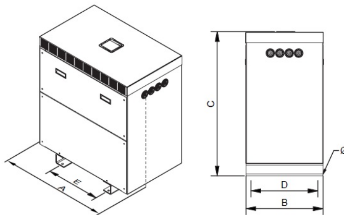
Dimensiones (AxBxCxDxE): 985x675x1310x475x470 mm 18Ø
