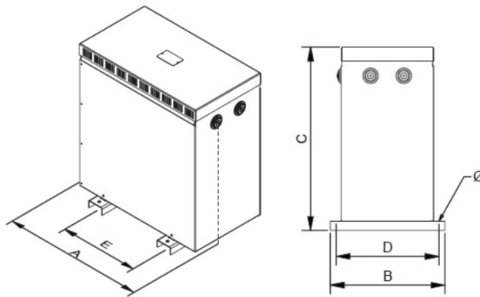
Dimensiones (AxBxCxDxE): 789x545x965x500x415 mm 13Ø
