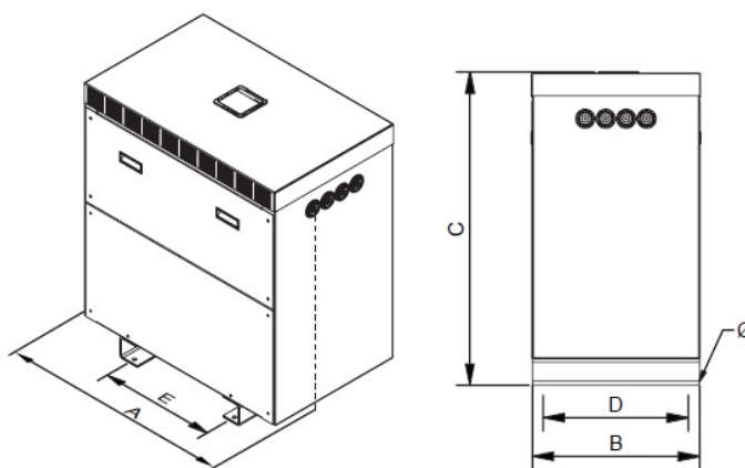
Dimensiones (AxBxCxDxE): 789x545x965x500x415 mm 13Ø
