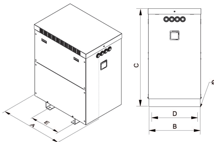
Dimensions (AxBxCxDxE): 789x545x965x500x415 mm 13Ø
