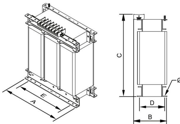
Dimensiones (AxBxCxDxE): 1070x550x1220x460x690 mm 17Ø
