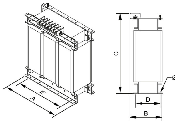
Dimensions (AxBxCxDxE): 1070x550x1220x460x690 mm 17∅
