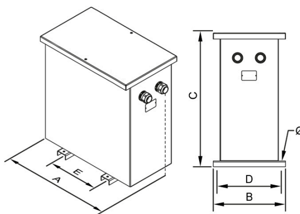
Dimensiones (AxBxCxDxE): 970x625x1150x500x426 mm 12Ø
