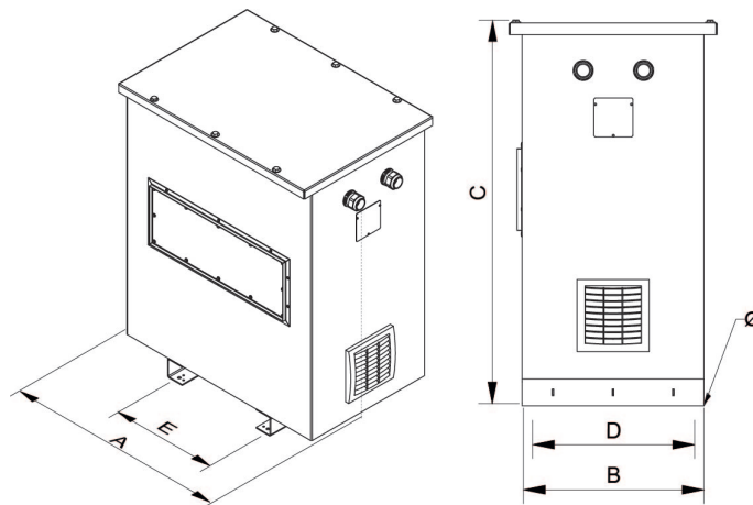
Dimensions (AxBxCxDxE): 1950x1100x1800x900x790 mm 20φ
