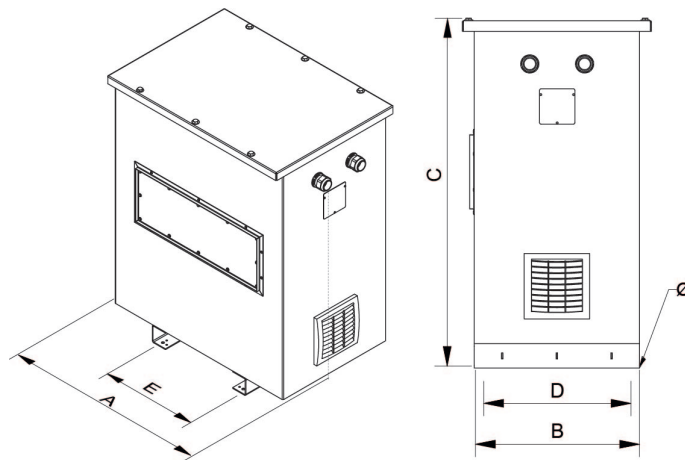
Dimensions (AxBxCxDxE): 970x625x1150x500x426 mm 12∅
