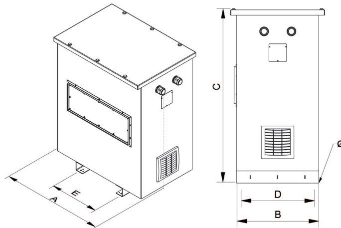
Dimensions (AxBxCxDxE): 970x625x1150x500x426 mm 12 \emptyset
