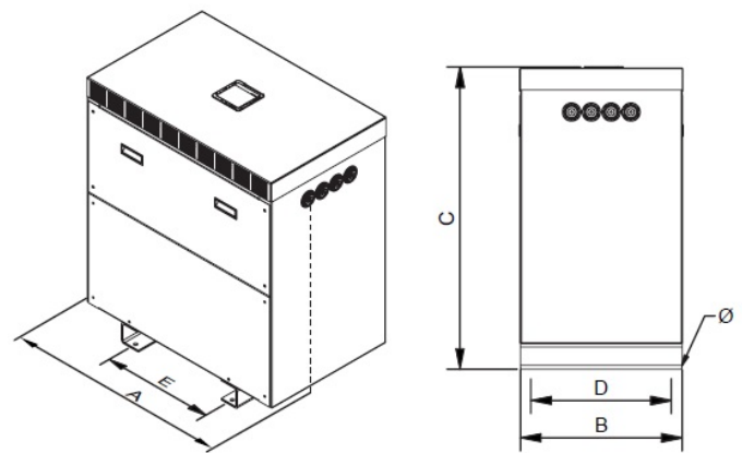
Dimensiones (AxBxCxDxE): 970x670x1250x582x470 mm 18φ
