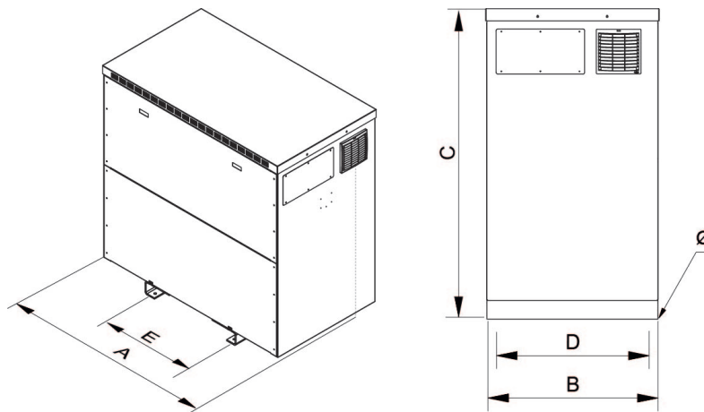
Dimensions (AxBxCxDxE): 1820x1000x1800x900x790 mm 20 \phi
