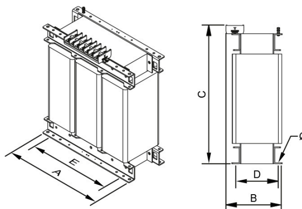
Dimensiones (AxBxCxDxE): 1070x550x1220x460x690 mm 17
