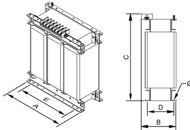
Dimensions (AxBxCxDxE): 670x310x580x170x426 mm 13
