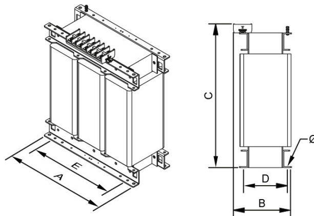
Dimensions (AxBxCxDxE): 670x330x580x190x426 mm 13
