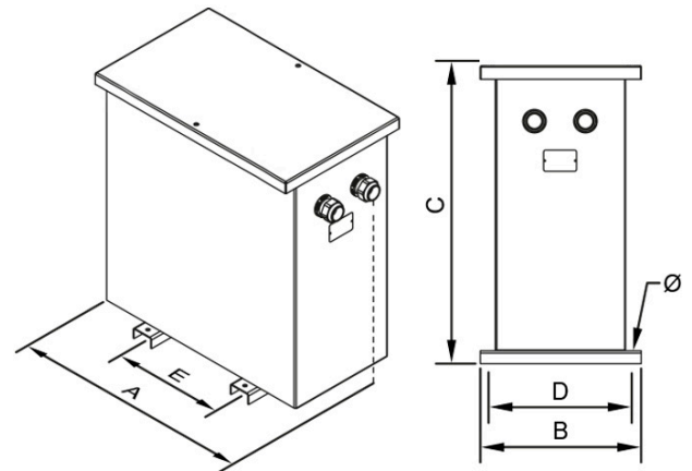
Dimensiones (AxBxCxDxE): 1550x1000x1750x806x684 mm 18Ø
