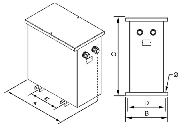
Dimensiones (AxBxCxDxE): 970x625x1150x500x426 mm 12∅
