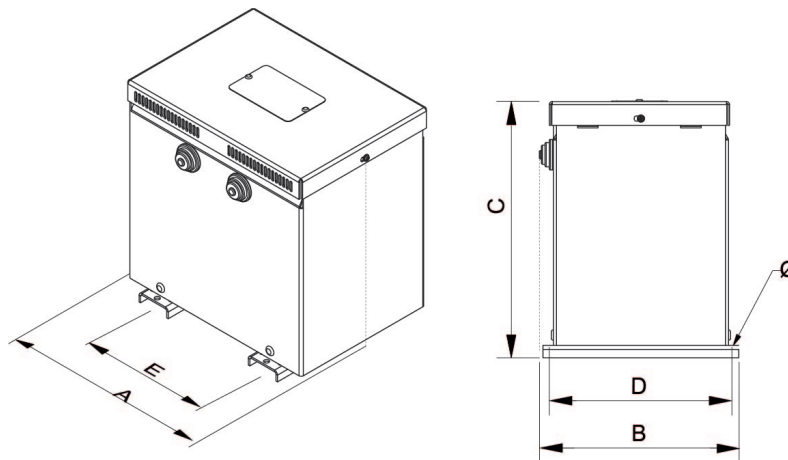
Dimensions (AxBxCxDxE): 240x190x250x180x150 mm 6
