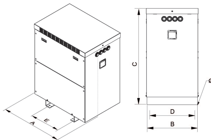
Dimensions (AxBxCxDxE): 970x670x1250x582x470 mm 18
