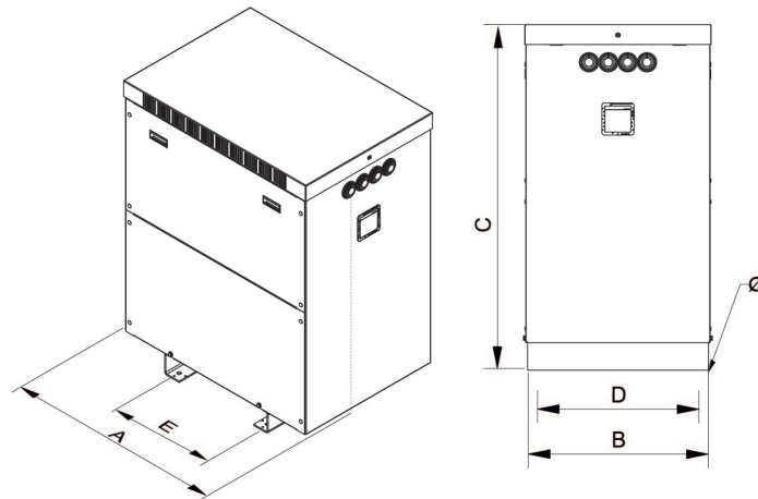
Dimensions (AxBxCxDxE): 795x550x970x500x415 mm 12
