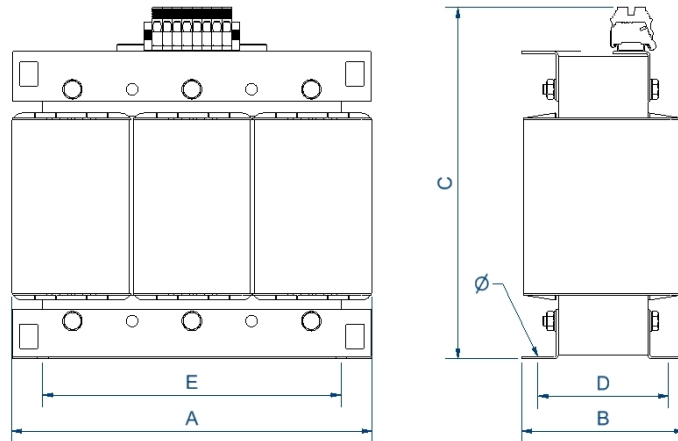
Dimensions (AxBxCxDxE): 360x164x353x142x300 mm 11
