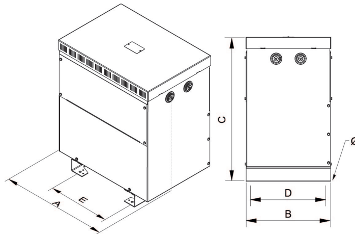
Dimensions (AxBxCxDxE): 458x340x500x300x300 mm 12Ø
