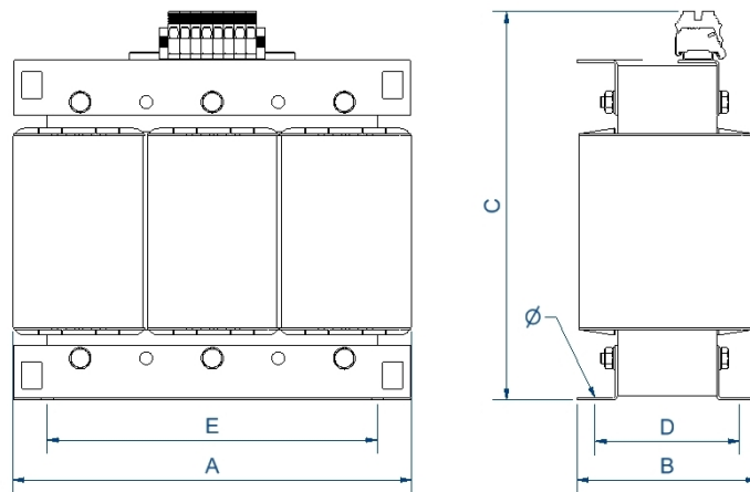
Dimensions (AxBxCxDxE): 360x164x353x142x300 mm 11Ø
