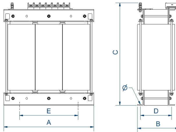
Dimensions (AxBxCxDxE): 670x360x690x230x426 mm 13Ø
