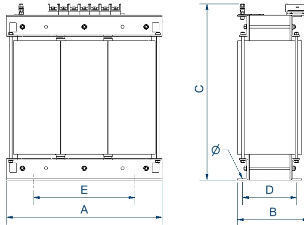
Dimensions (AxBxCxDxE): 785x550x880x460x472 mm 17Ø
