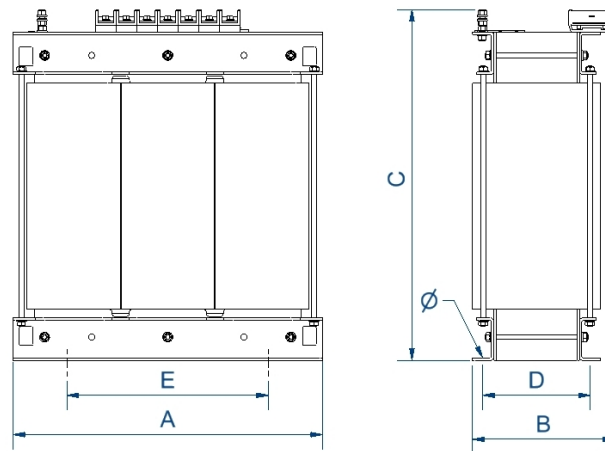
Dimensions (AxBxCxDxE): 1016x550x1080x460x690 mm 17
