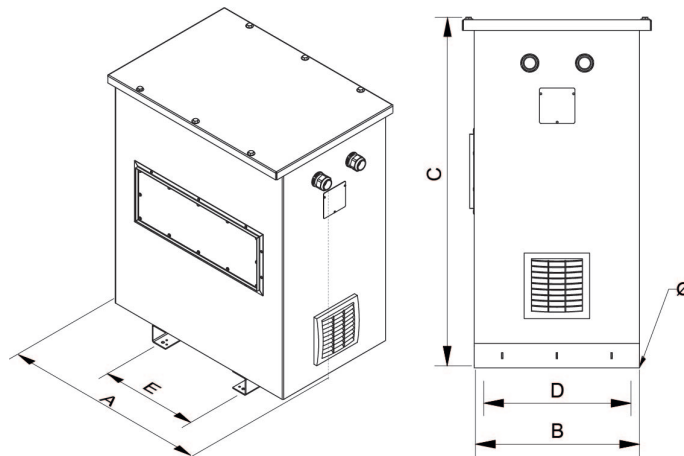
Dimensions (AxBxCxDxE): 694x413x764x370x350 mm 11Ø
