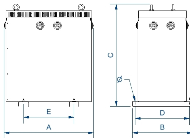
Dimensiones (AxBxCxDxE): 458x340x500x300x300 mm 12Ø
