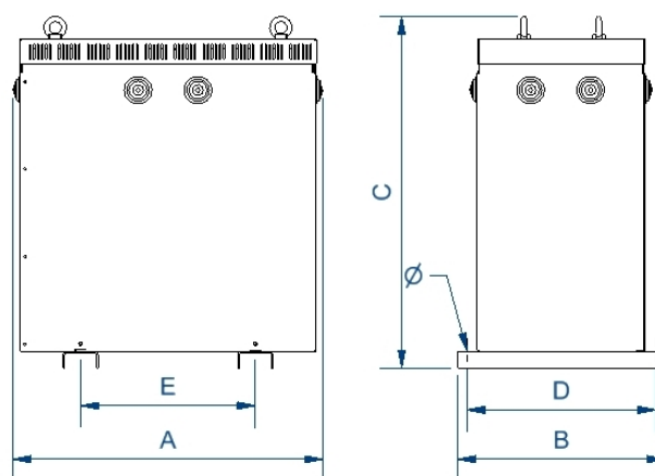
Dimensions (AxBxCxDxE): 385x260x384x245x250 mm 6Ø
