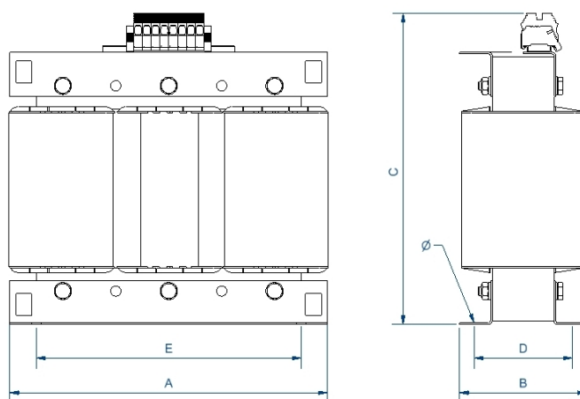
Dimensions (AxBxCxDxE): 260x118x253x94x200 mm 9Ø
