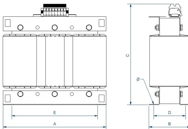
Dimensions (AxBxCxDxE): 470x190x419x156x350 mm 11Ø
