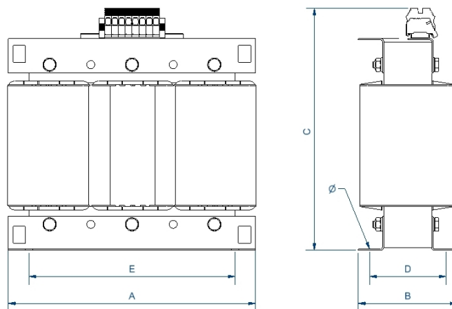
Dimensions (AxBxCxDxE): 530x260x480x154x400 mm 11Ø
