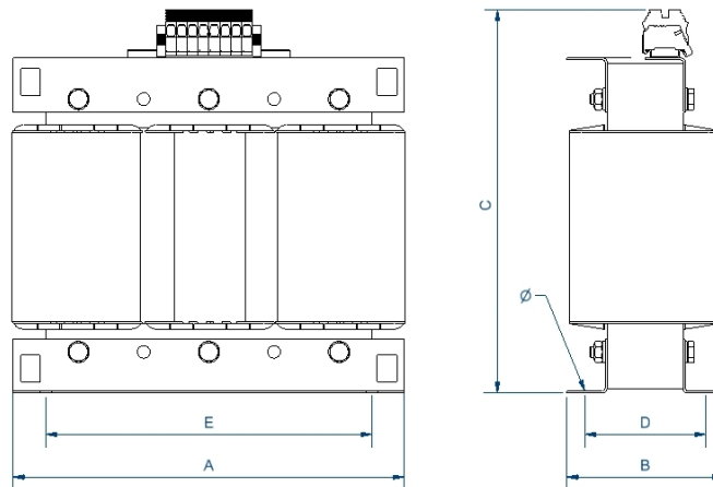
Dimensions (AxBxCxDxE): 530x310x480x204x400 mm 11Ø
