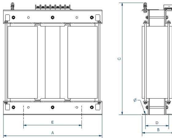
Dimensions (AxBxCxDxE): 740x290x580x170x426 mm 13Ø
