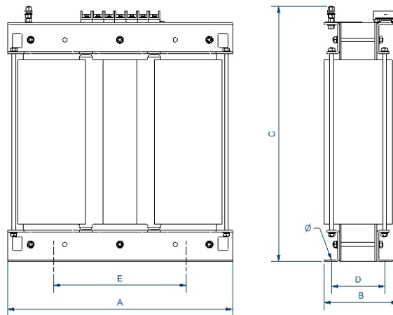
Dimensions (AxBxCxDxE): 740x310x580x190x426 mm 13Ø
