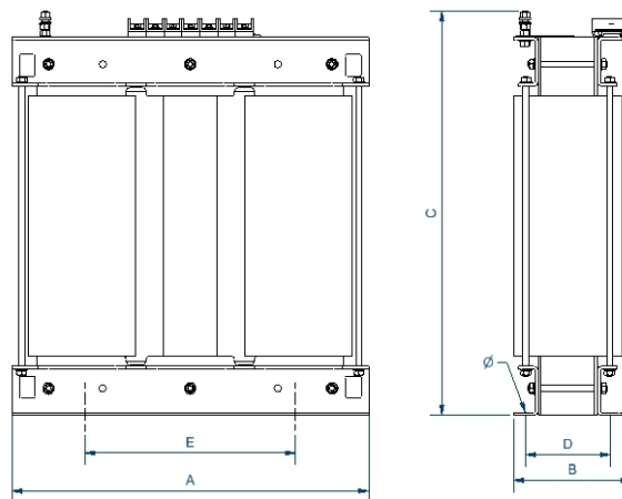
Dimensions (AxBxCxDxE): 785x550x880x460x472 mm 17Ø
