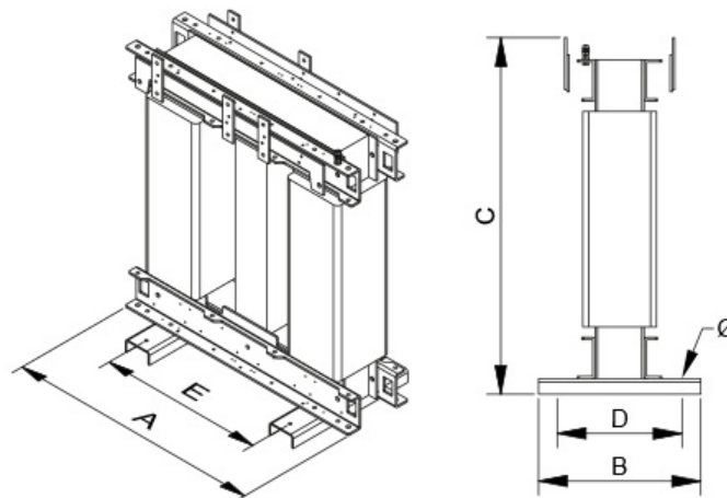
Dimensions (AxBxCxDxE): 785x550x880x460x472 mm 17Ø
