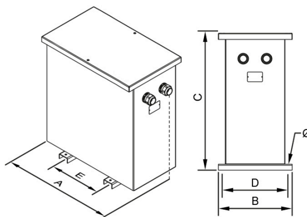
Dimensions (AxBxCxDxE): 510x362x689x320x250 mm 11Ø
