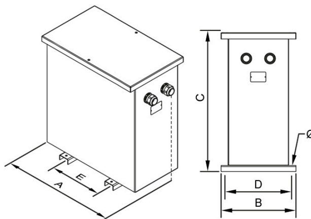
Dimensions (AxBxCxDxE): 970x625x1150x500x426 mm 12Ø
