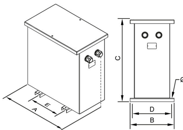
Dimensions (AxBxCxDxE): 694x413x764x370x350 mm 110
