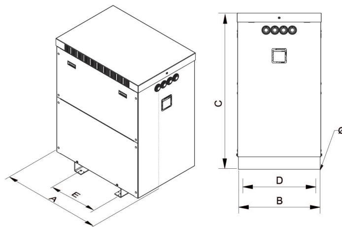
Dimensiones (AxBxCxDxE): 1200x760x1555x672x690 mm 18 \phi
