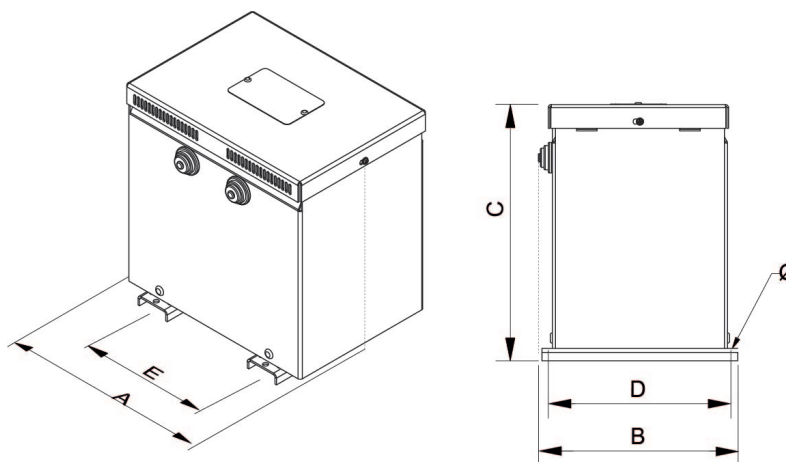
Dimensions (AxBxCxDxE): 235x190x250x180x150 mm 6Ø
