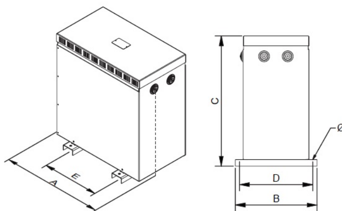
Dimensions (AxBxCxDxE): 235x190x250x180x150 mm 6Ø
