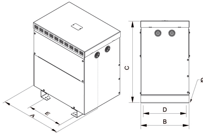
Dimensions (AxBxCxDxE): 521x415x644x375x345 mm 12Ø
