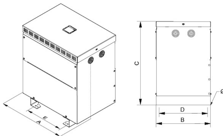
Dimensions (AxBxCxDxE): 521x415x644x375x345 mm 12Ø
