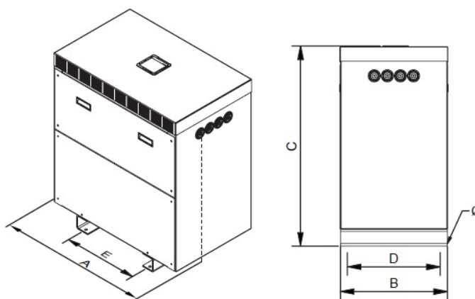
Dimensions (AxBxCxDxE): 990x685x1255x582x470 mm 18Ø
