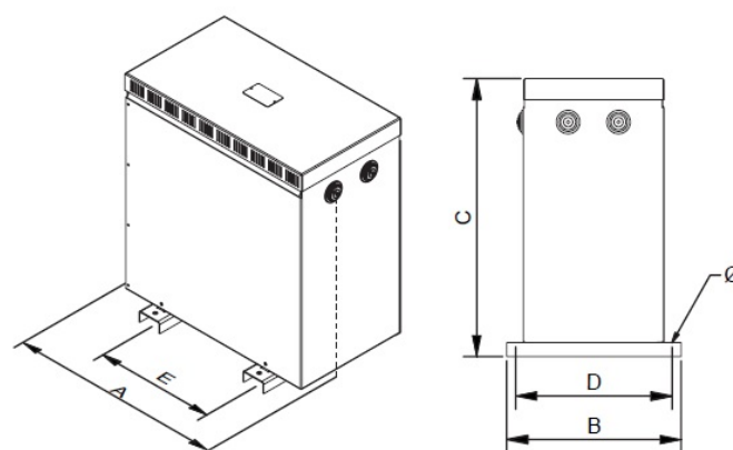
Dimensiones (AxBxCxDxE): 451x340x501x300x300 mm 12Ø
