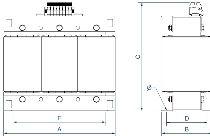
Dimensions (AxBxCxDxE): 420x190x421x162x350 mm 11Ø
